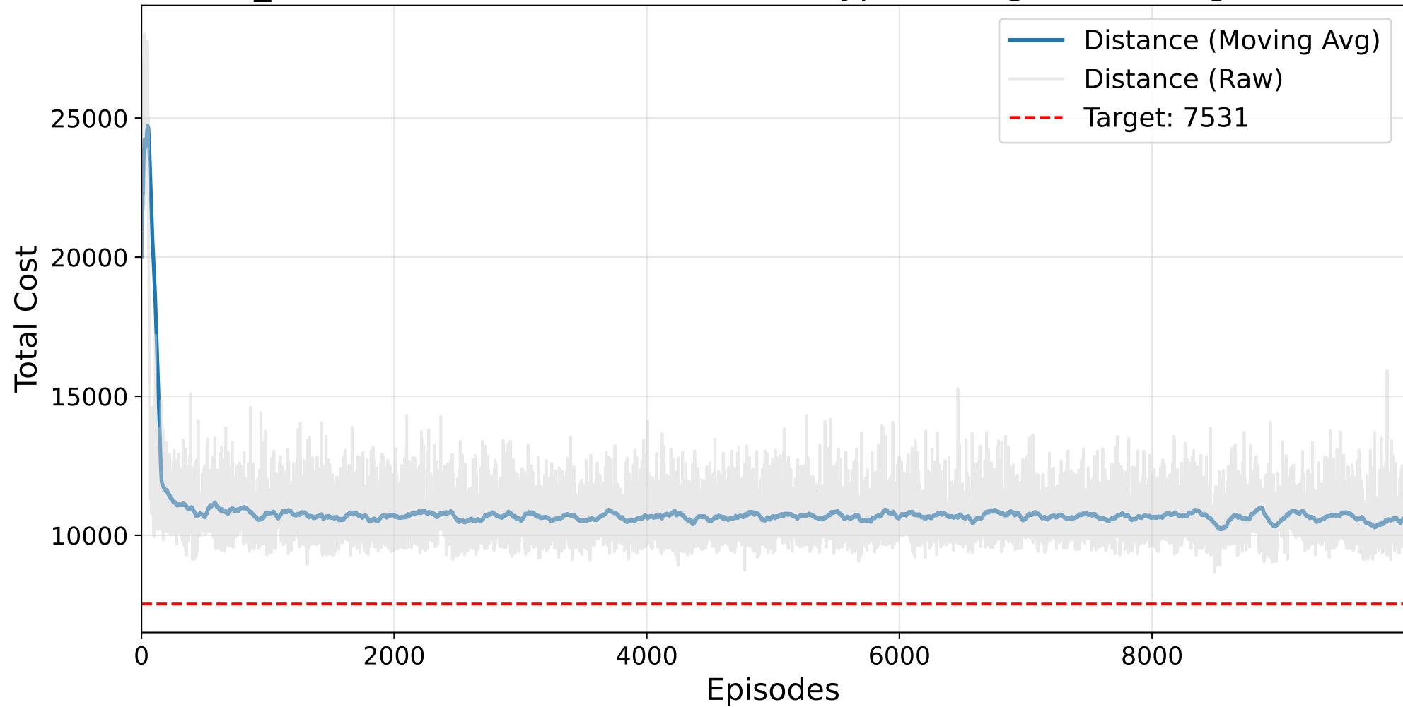
Final NO_BAYESIAN Masked AutoRL-SOP (HyperTuningSK) Training - ft53.1.sop
